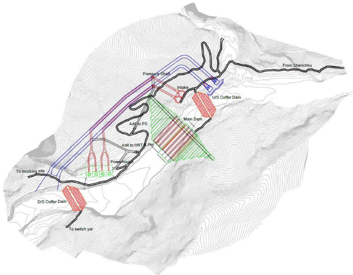
Figure 1: Project layout
