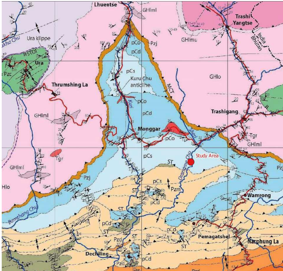
Figure 2: Project location regional geologic map
