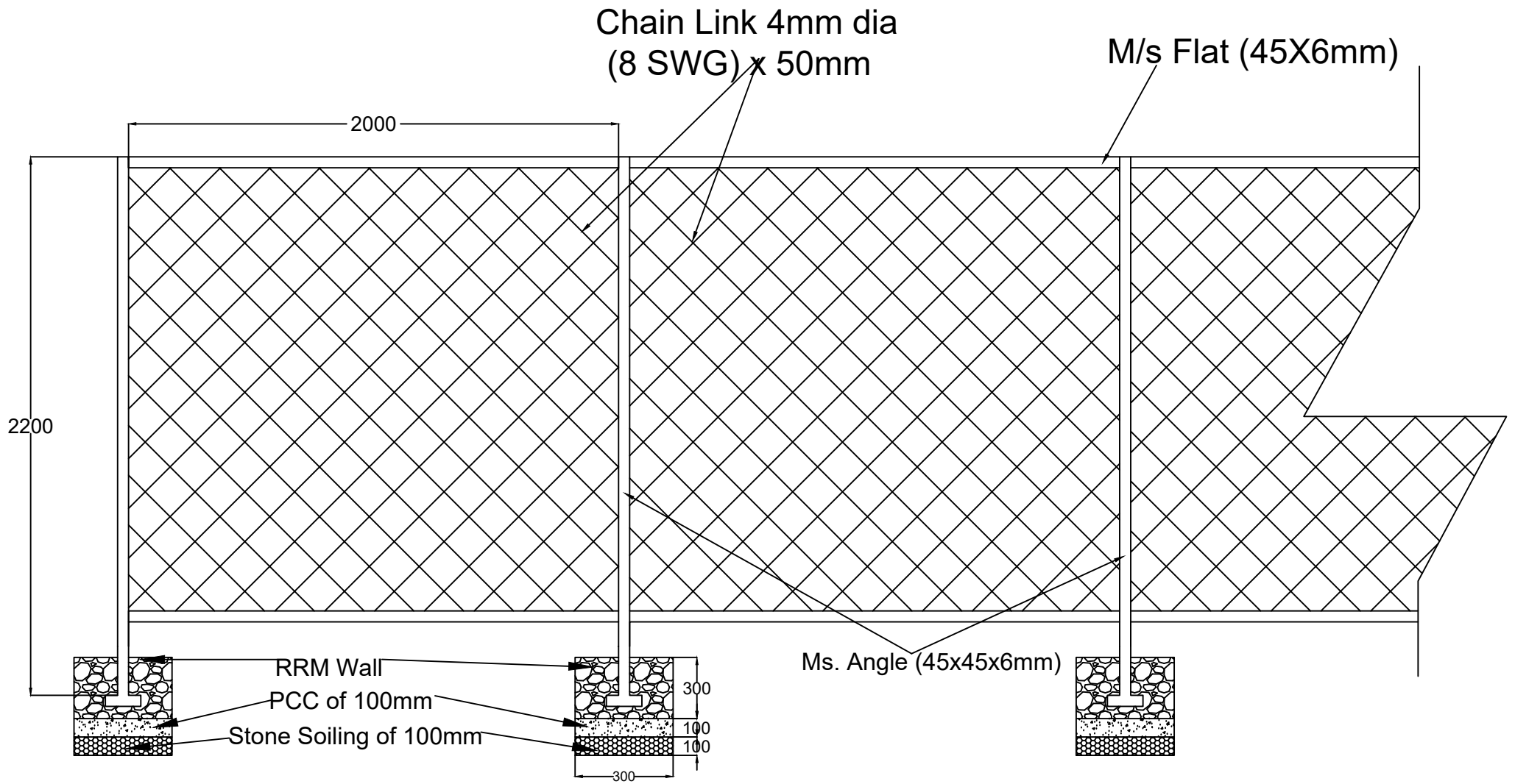
Typical Drawing of Chain Link Fencing
