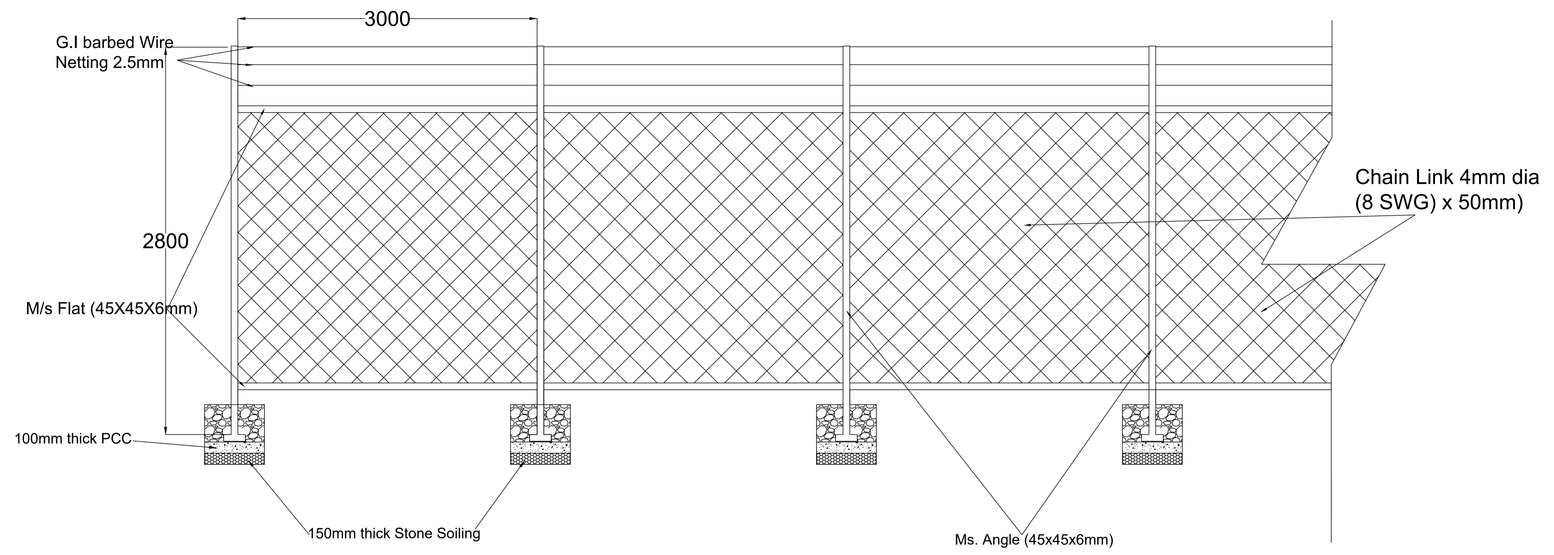
TYPICAL DRAWING FOR CHAINLINK FENCING
