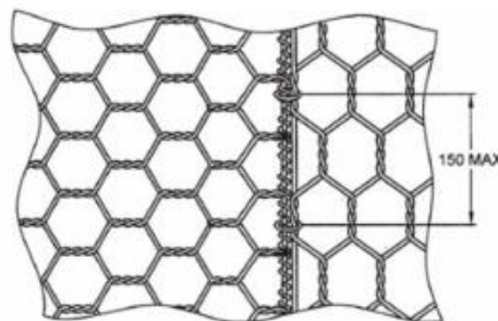
Figure 4 Rings for joining adjacent panels instead or with lacing wire
