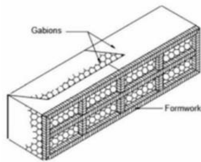
a) Temporary Formwork
