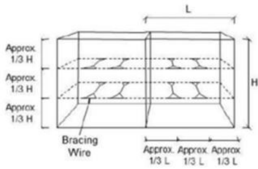
Figure 5 Bracing wire details for 1 m deep gabion crates
