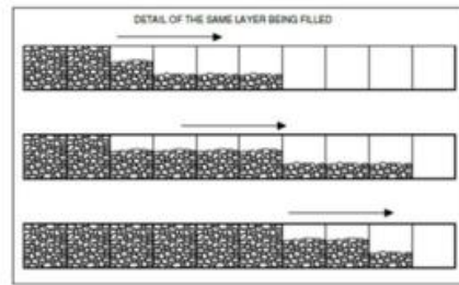
Figure 6 Filling pattern of gabion boxes
