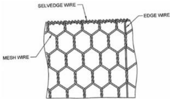
Figure 2 Mesh wire, Selvedge and Edge wire
