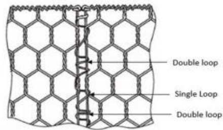
Figure 3 Lacing Wire for tying adjacent panels in single and double loop fashion
