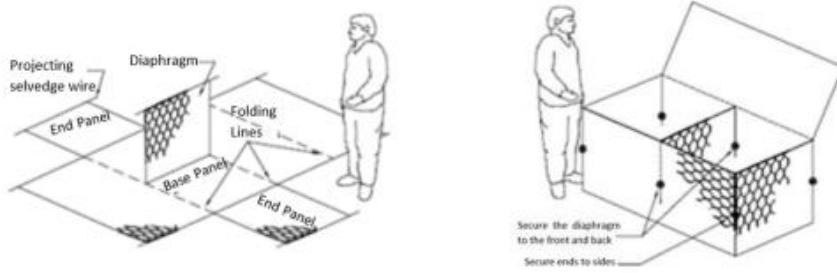
Figure 1 (a) and (b) Gabion installation
