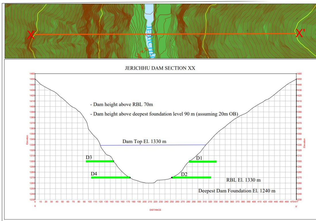
Figure 6: Section of the dam axis with the location of the drifts
