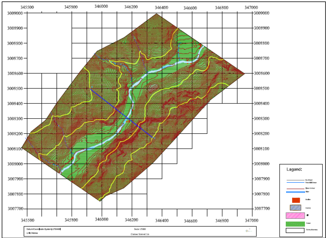
Figure 1: Dam Axis
