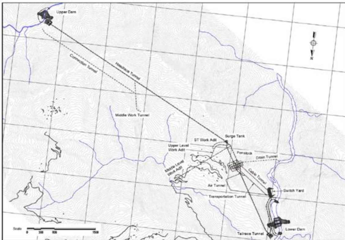
Figure 2: Project Layout
