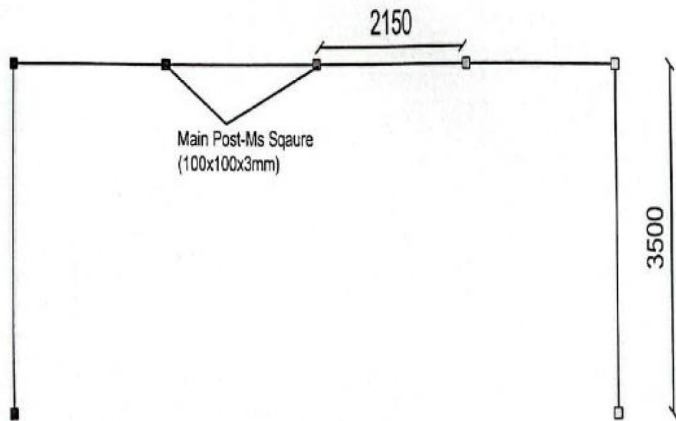
LAYOUT PLAN
