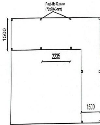
LAYOUT PLAN
