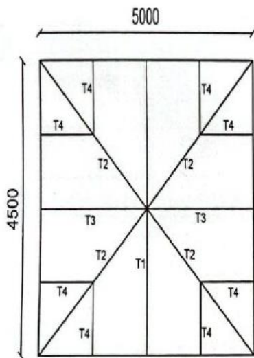
TRUSS LAYOUT
