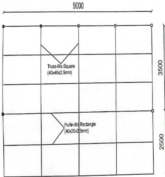
TRUSS LAYOUT
