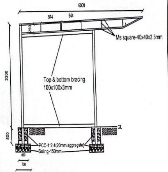
POST & TRUSS SECTION
