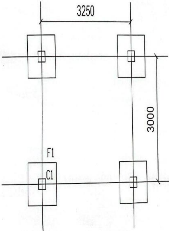
FOUNDATION LAYOUT PLAN
