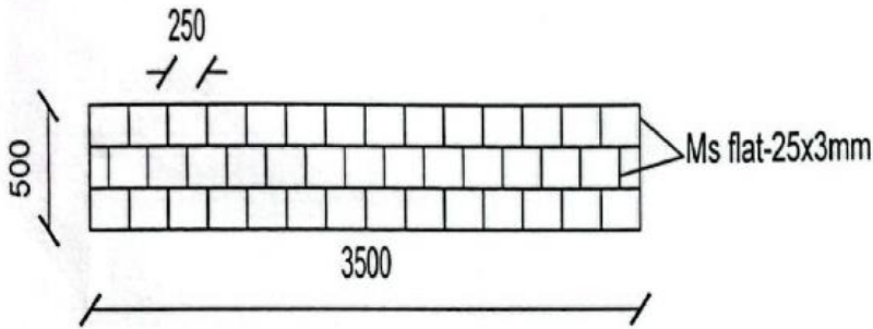
Ventilation Grill
