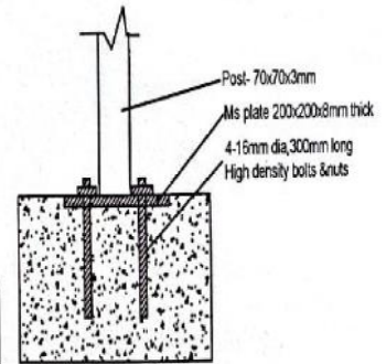
BASE PLATE & ANCHOR DETAIL
