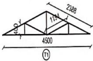
TRUSS LAYOUT
