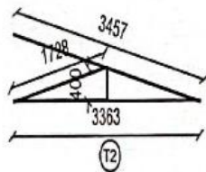
PURLIN LAYOUT
