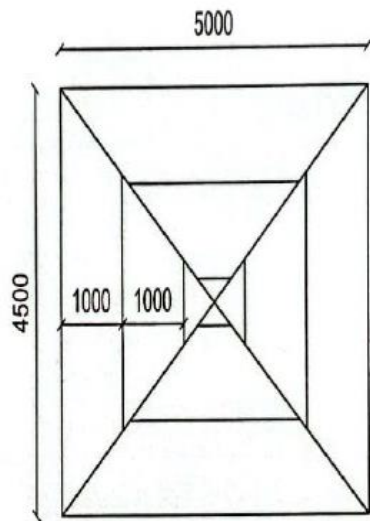
PURLIN LAYOUT
