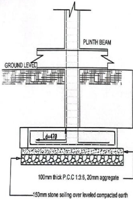
SECTIONAL ELEVATION FOR FOOTING
