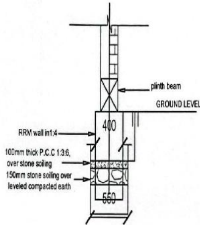
EXTERNAL WALL (250mm) FOUNDATION
