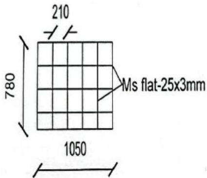
Window Grill
