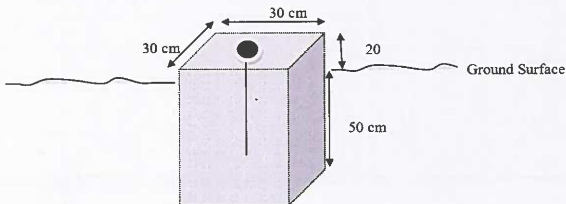
Figure 2: Ground Control Point/Block specifications
